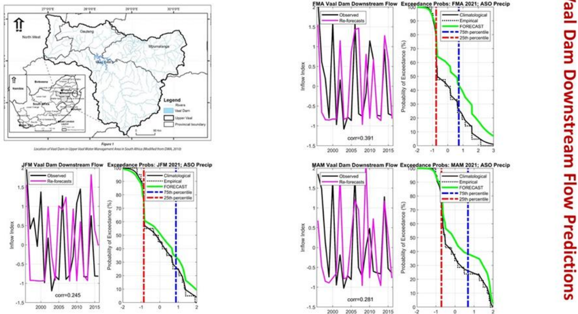
Figure 3.3 The first Vaal Dam seasonal forecasts of the University of Pretoria, November 2020.
