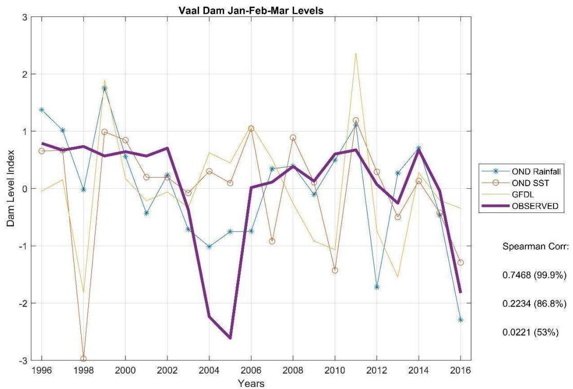
Figure 2 7 JFM dam level predictions, using antecedent (OND) rainfall conditions, OND SST and JFM rainfall forecasts from the GFDL climate model. The correlations and their level of statistical significance are listed in the same order from top to bottom as shown in the key.
