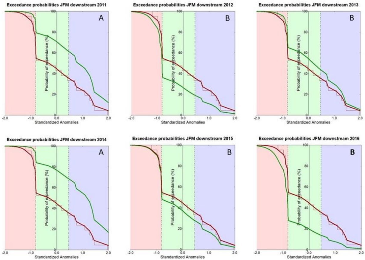
Figure 4.3 As for Figure 4.2, but for JFM downstream flow.
